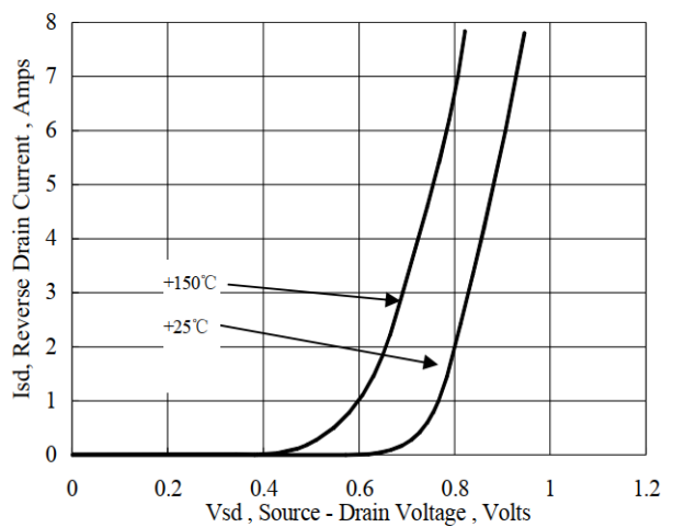
Fig 6 Body-Diode Characteristics
